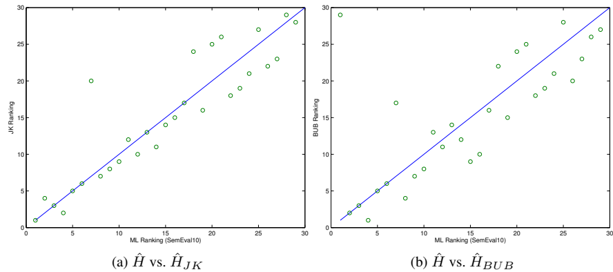
Figure 4: Discrepancy in rankings as function of the predicted number of classes.
