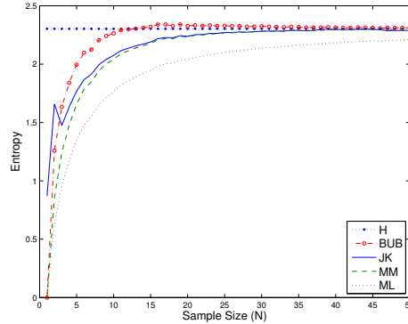
Figure 1: The estimated and true entropy for uniform distribution.
