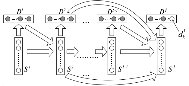
Figure 1: An ISBN for estimating P(d_k^t | h(t, k)) .
