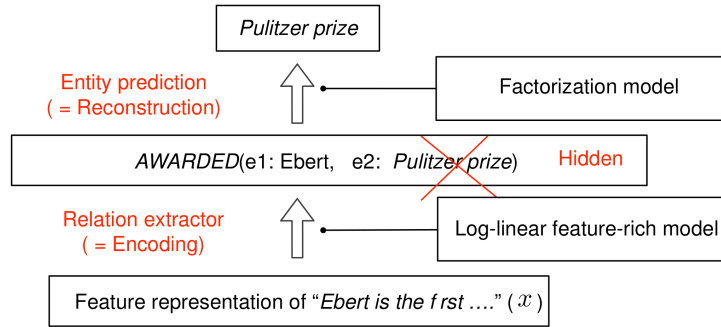
Figure 1: Inducing relations with discrete-state autoencoders.
